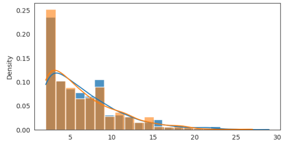
Predictive distribution of time until the next recession
