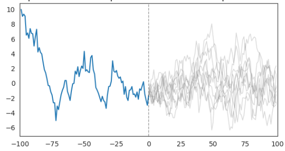
Initial path and future paths simulated from posterior draws
